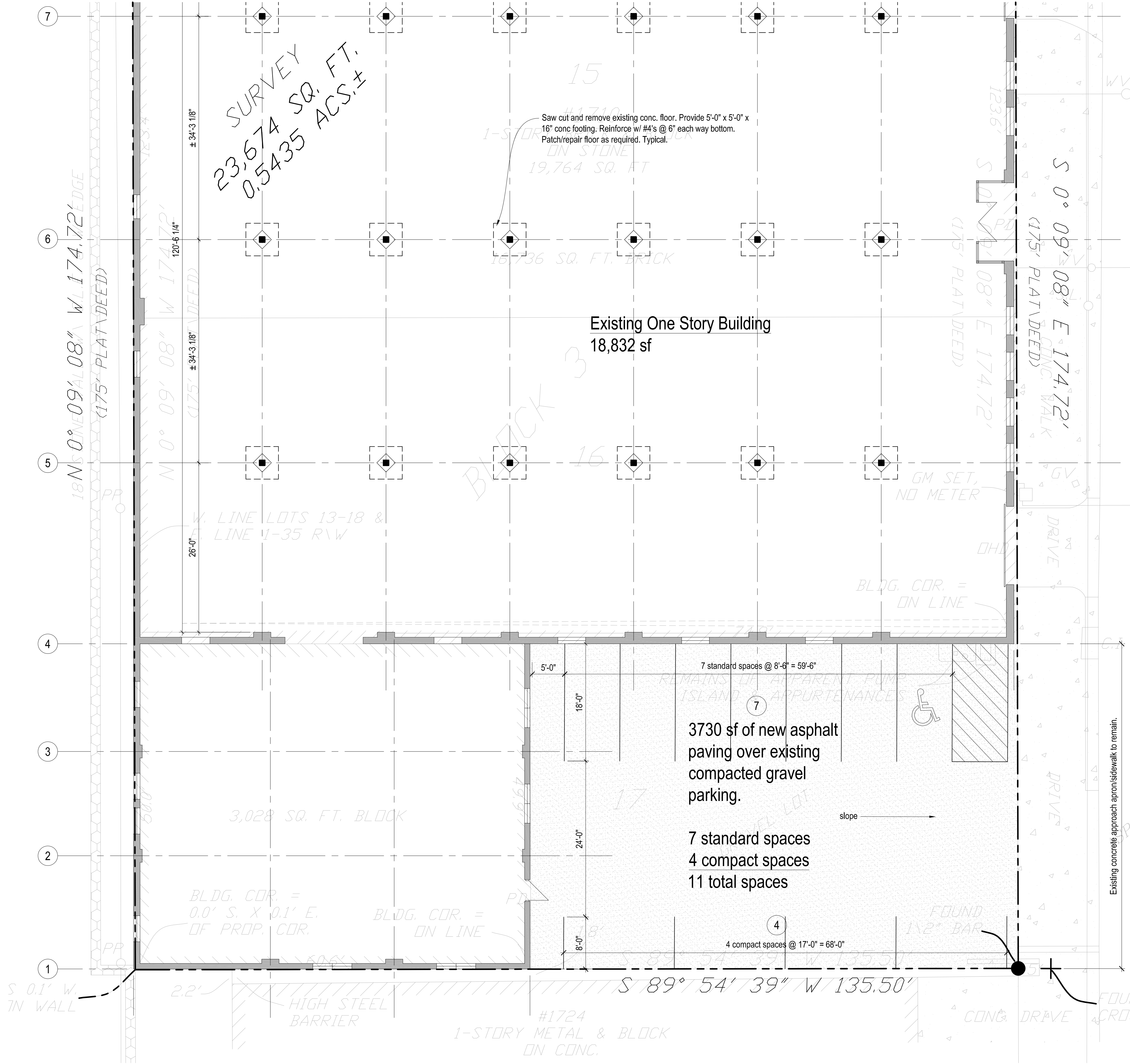
A1 Partial Site / Parking Plan 1/8" = 1'-0"
